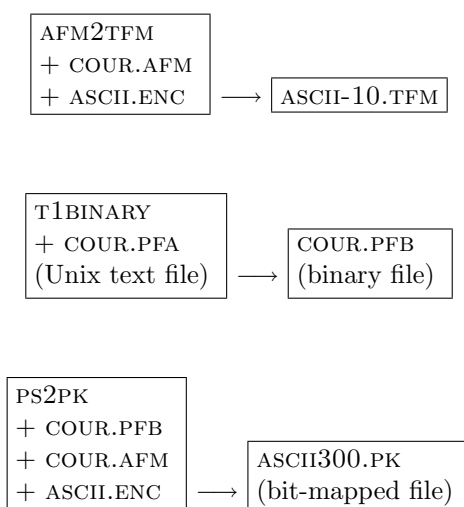
Figure 1: Sequence of file changes to generate ASCII-10.TFM and ASCII300.PK.
